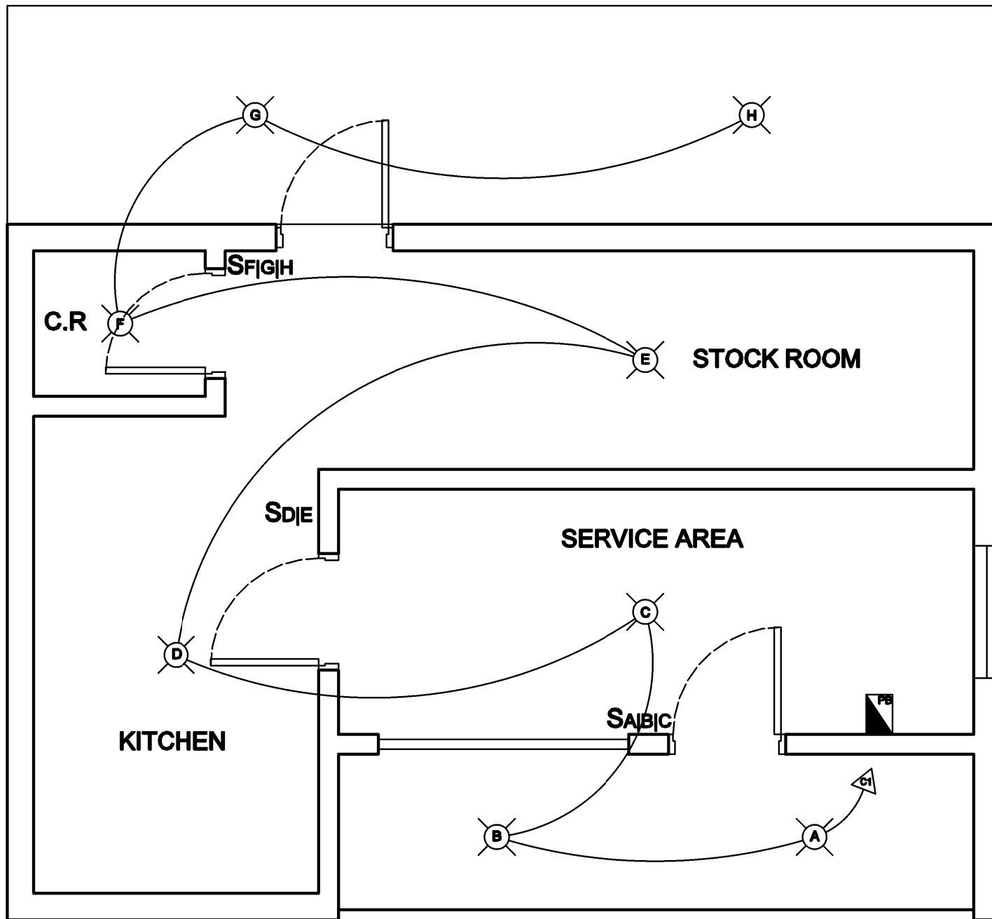
ELECTRICAL LIGHTNING LAY OUT
